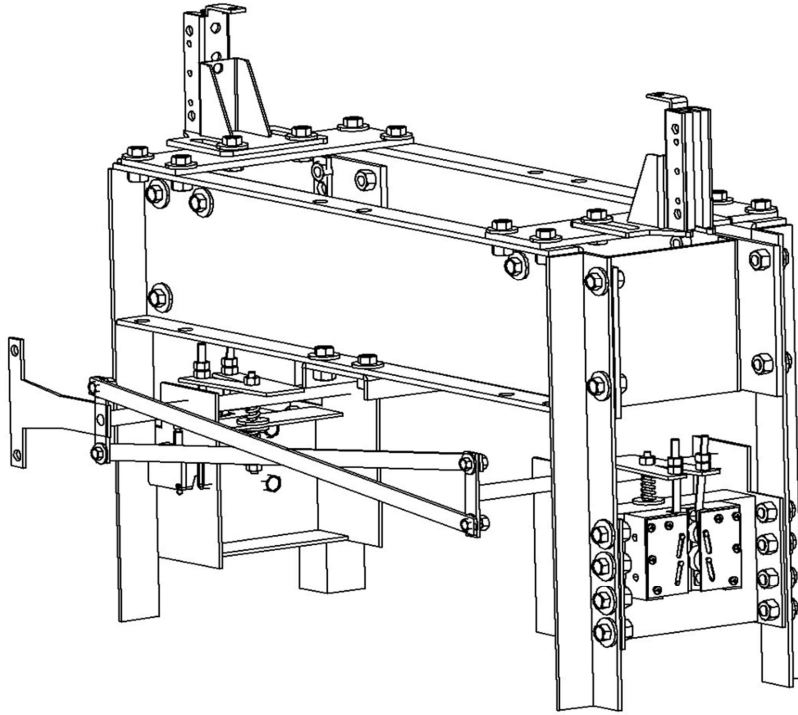
Safety gear synchronisation bar
